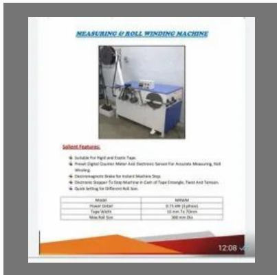
Elastic Tape Roll Winding Machine
